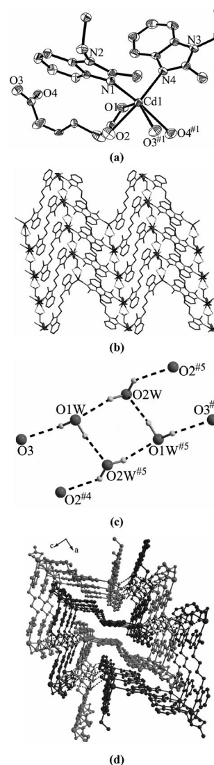
Figure 9. (a) ORTEP diagram showing the coordination environment for the Cd atom in 9 . (b) The infinite 2-D wavelike layer. (c) View of the (H_2O)_4 cluster. (d) The packing diagram of 9 (dashed lines represent hydrogen bonds).
